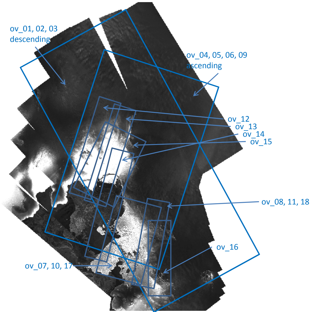
Thwaites and Pine Island Glaciers 2007 Velocity Product (ov_*) locations
