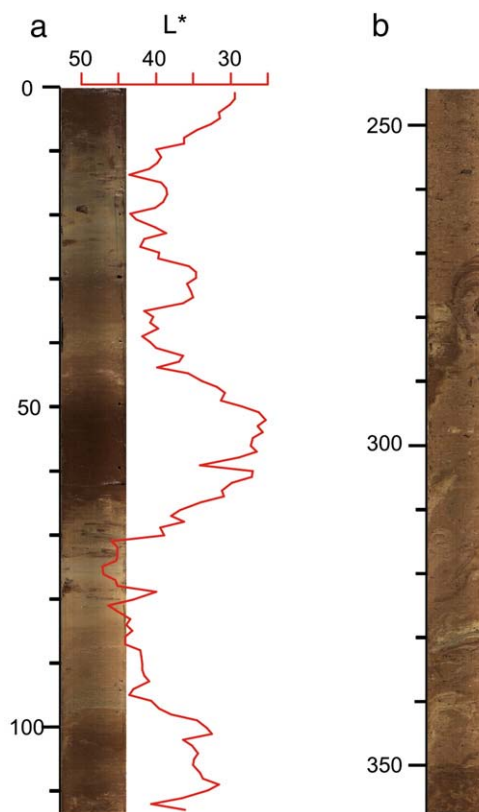
Fig. 3. Photographic fragments of HLY0503-8JPC that exemplify (a) normal stratification, with brown/gray interlamination approximated by L^* , and (b) interval with gravity-flow sedimentary structures between 270 to 350 cm.
