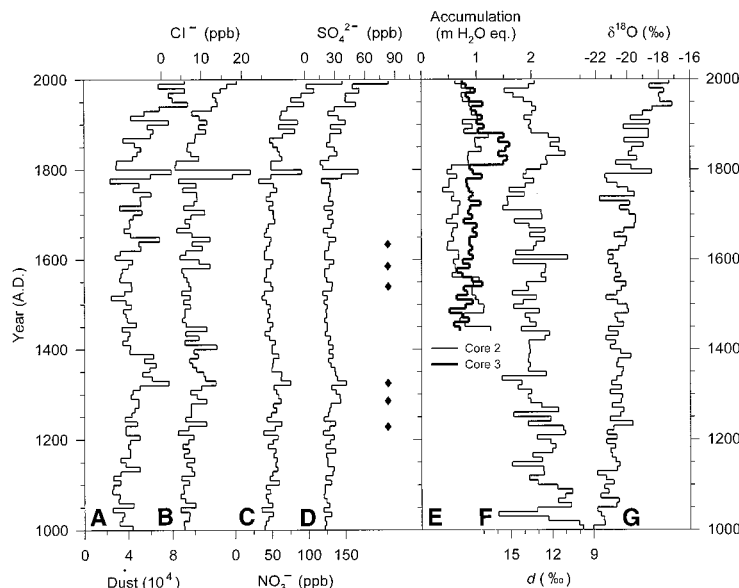
Fig. 5 (left). Decadal values of (A) dust, (B) \text{Cl}^- , (C) \text{NO}_3^- , (D) \text{SO}_4^{2-} , (E) net accumulation (for cores 2 and 3), (F) deuterium-excess ( d ), and (G) \delta^{18}\text{O} are shown for the last 1000 years. Accumulation rates are reconstructed after Bolzan (34) and Reeh (35). Diamonds indicate correlative increases in these parameters that may reflect six monsoon failures that were much less dramatic than that of 1790 to 1796.
